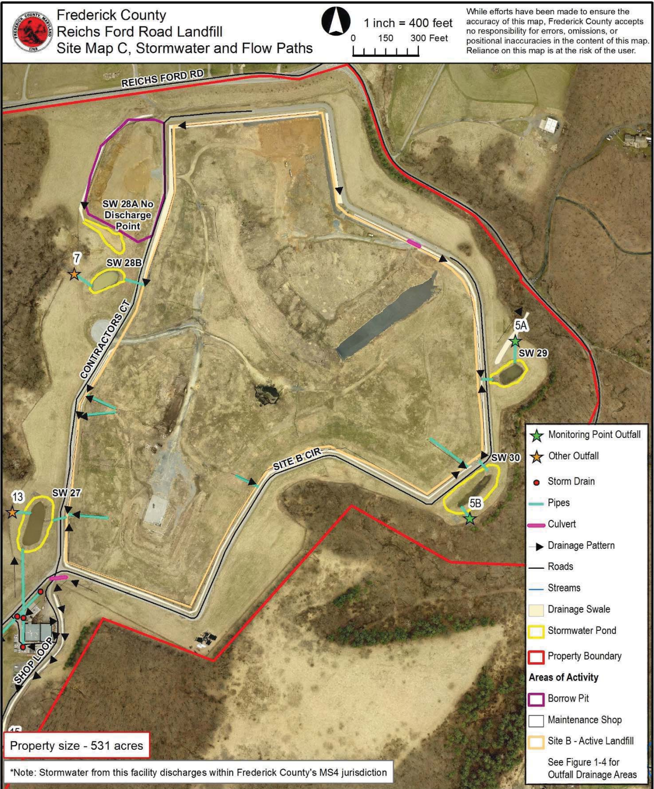
Figure 1-10. Site Map C: Stormwater detail for Site B active landfill, borrow pit.
